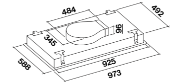
Slim motor (only onboard)
