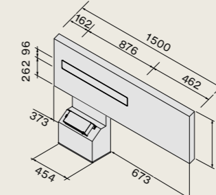
Air Wall 150 Module paneel 150 cm links afzuiging
