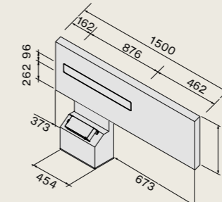
Air Wall 150 Module paneel 150 cm links afzuiging
